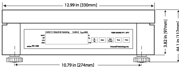
OUTLINE OF SCALE AND DIMENSIONS
